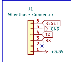
Connection to the wheelbase
