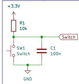
Switch debounce circuit (no software debouncing)
